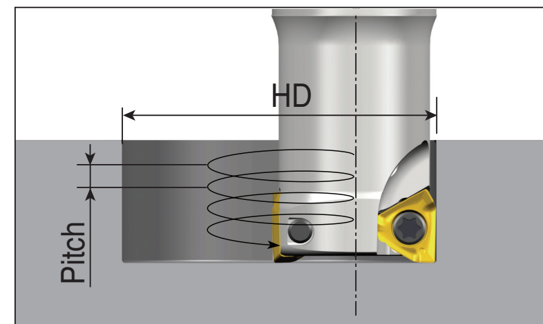
Helical ramping
