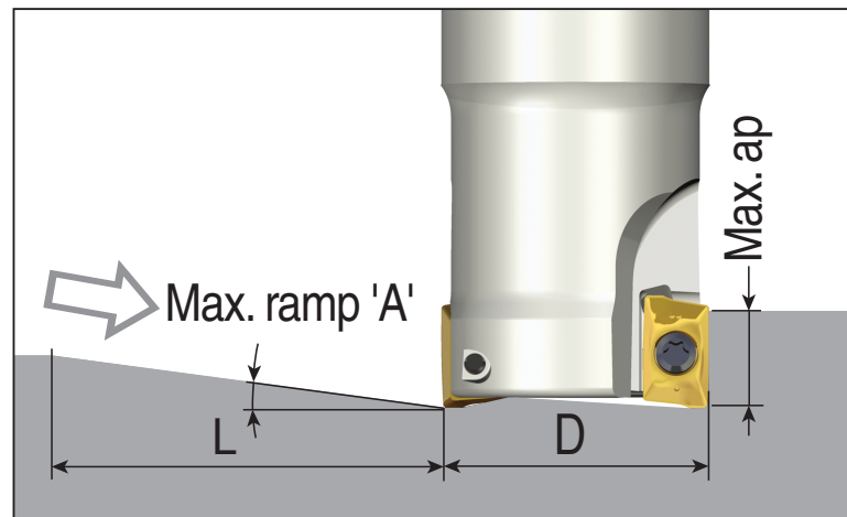
Straight ramping
