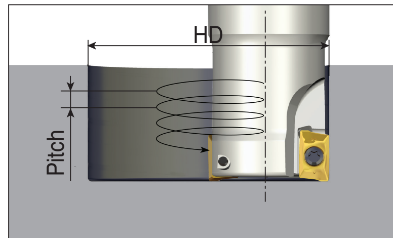
Helical ramping
