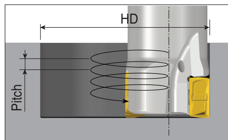
Helical ramping
