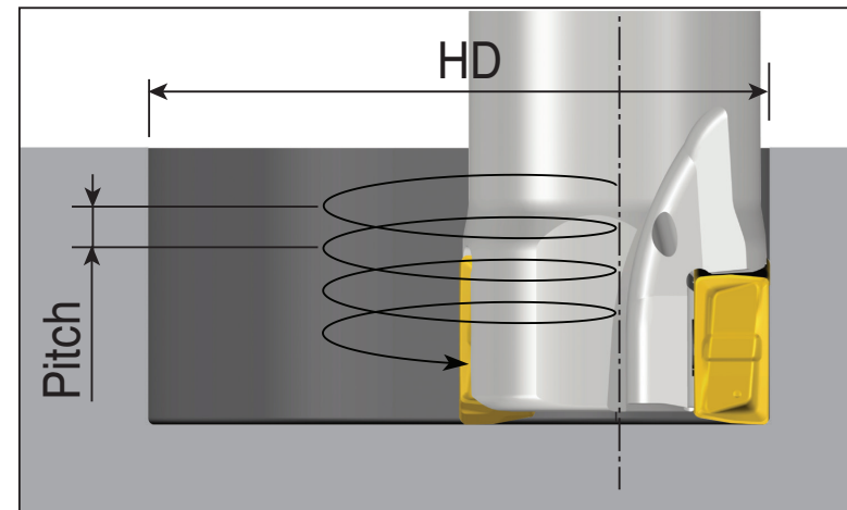
Helical ramping
